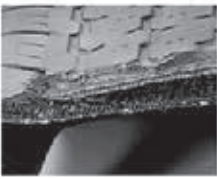
Belt Separation
