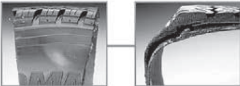
Sidewall Bubble - A bulge that appears on the outside of a tire is usually a sign of separation.
